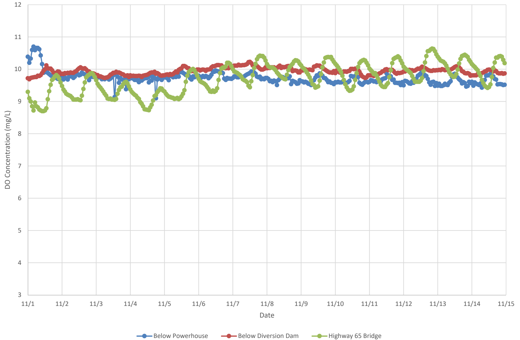
Hourly DO Concentrations (mg/L) with Camp Far West Powerhouse Not Operating, No Diversions Occurring, and Flows at Wheatland Gage (15-26cfs)
