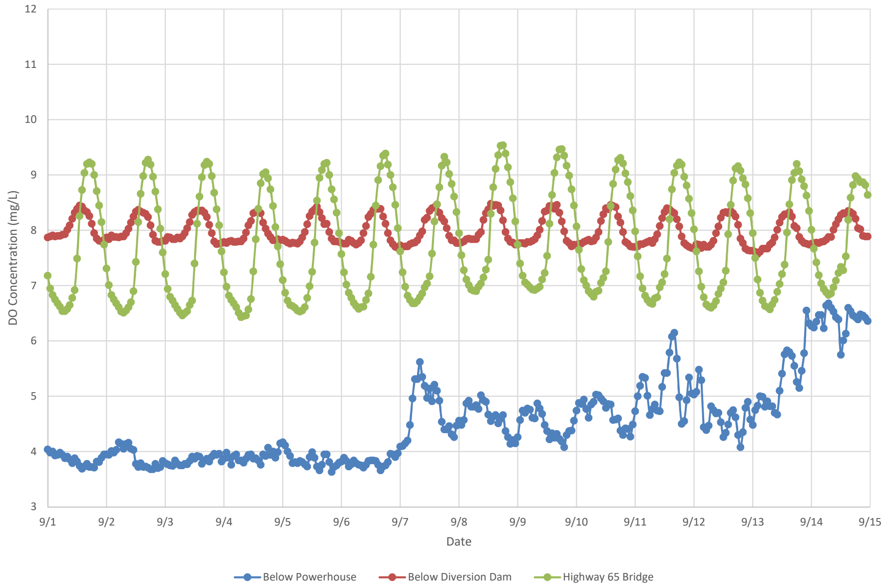
Hourly DO Concentrations (mg/L) with Camp Far West Powerhouse Operating (249-390cfs), Diversions Occurring (199-381cfs), and Flows at Wheatland Gage (13-31cfs)
