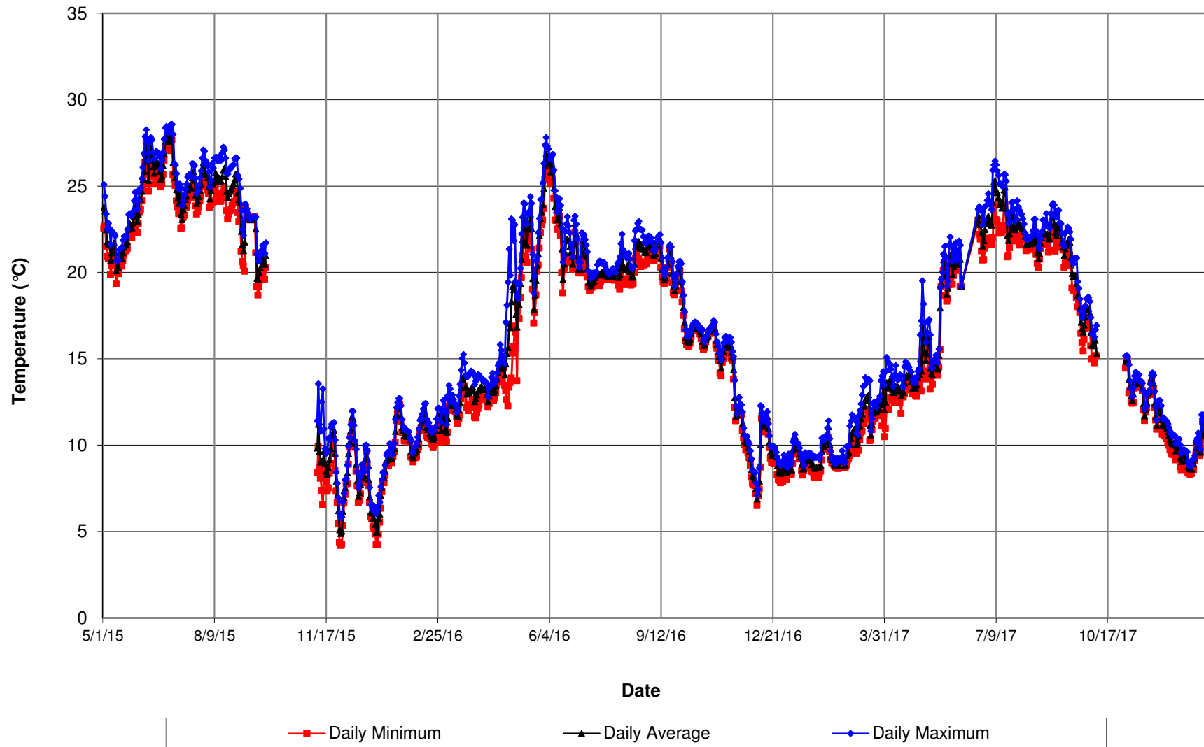
Bear River upstream of Feather River Daily Minimum, Average, and Maximum Water Temperature (°C) Note: Depending on flows this site can be backwatered by the Feather River
