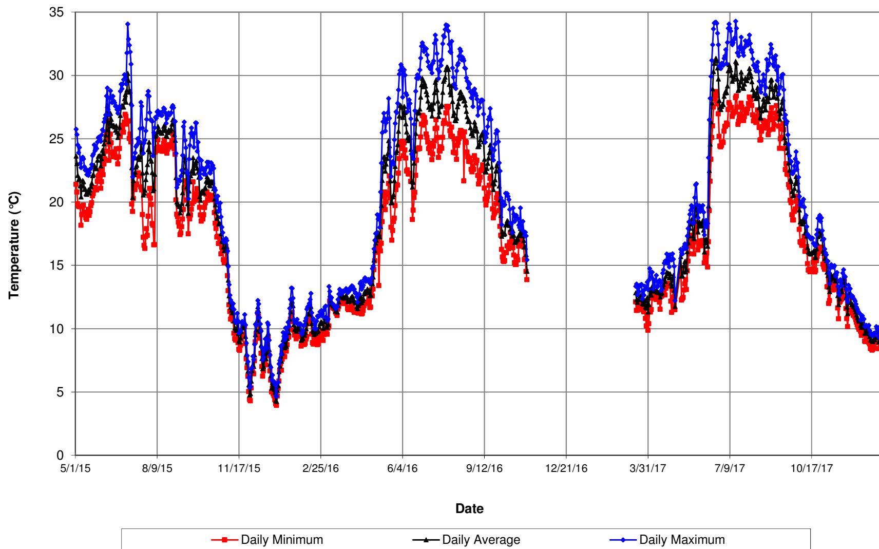
Bear River upstream of Pleasant Grove Bridge Daily Minimum, Average, and Maximum Water Temperature (°C)
