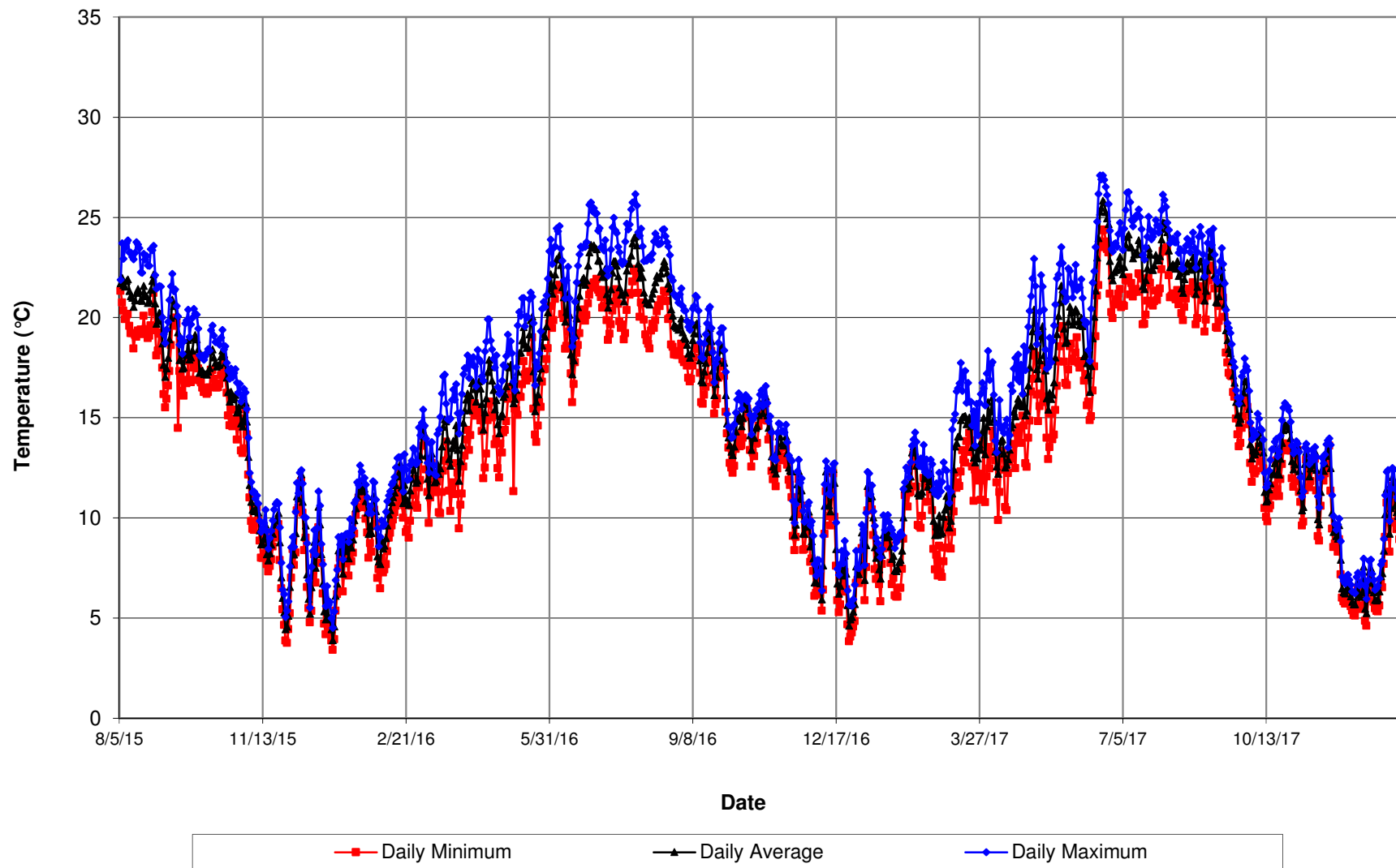
Rock Creek upstream of Camp Far West Reservoir Daily Minimum, Average, and Maximum Water Temperature (°C)
