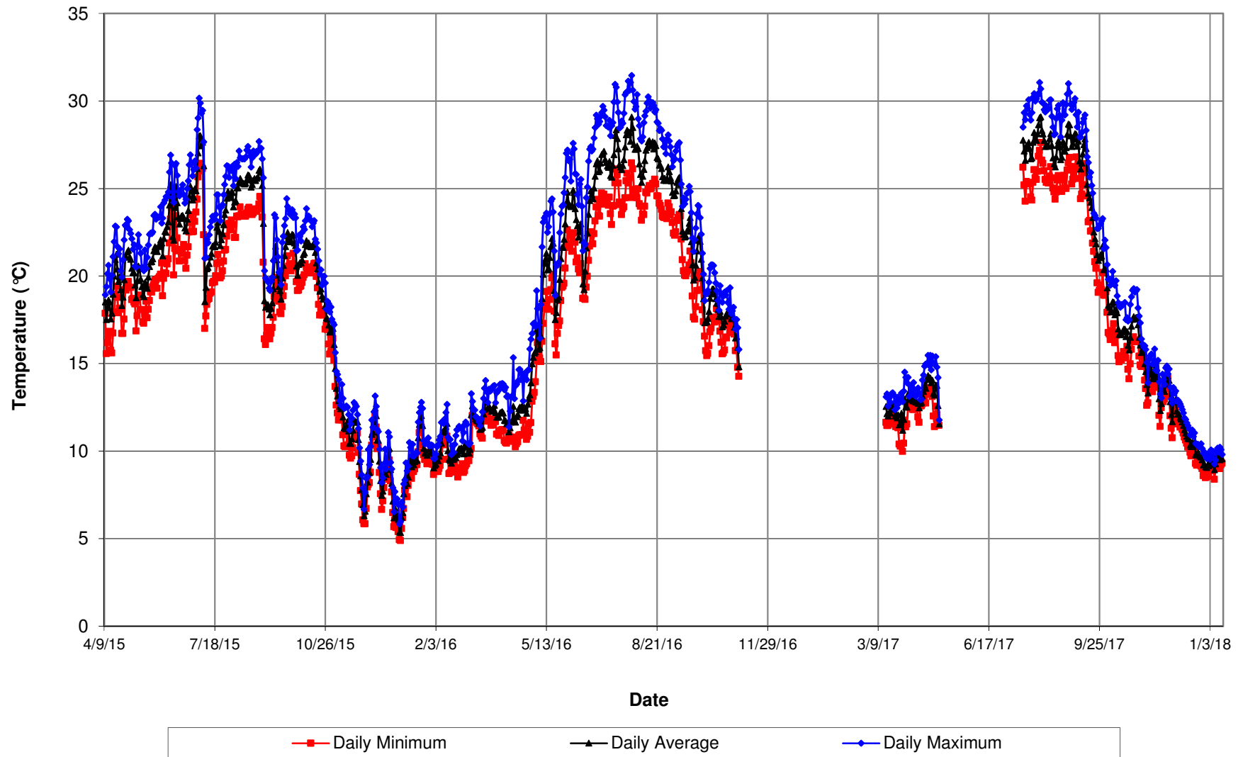
Bear River downstream of Highway 65 Bridge Daily Minimum, Average, and Maximum Water Temperature (°C)
