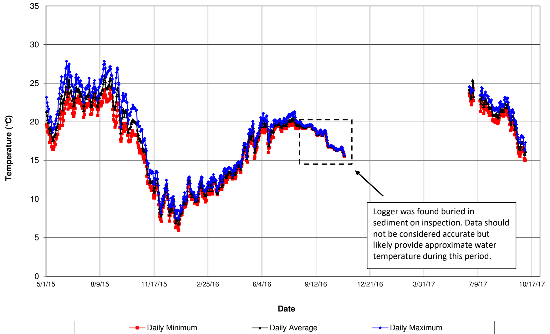
Feather River downstream of Bear River Daily Minimum, Average, and Maximum Water Temperature (°C)
