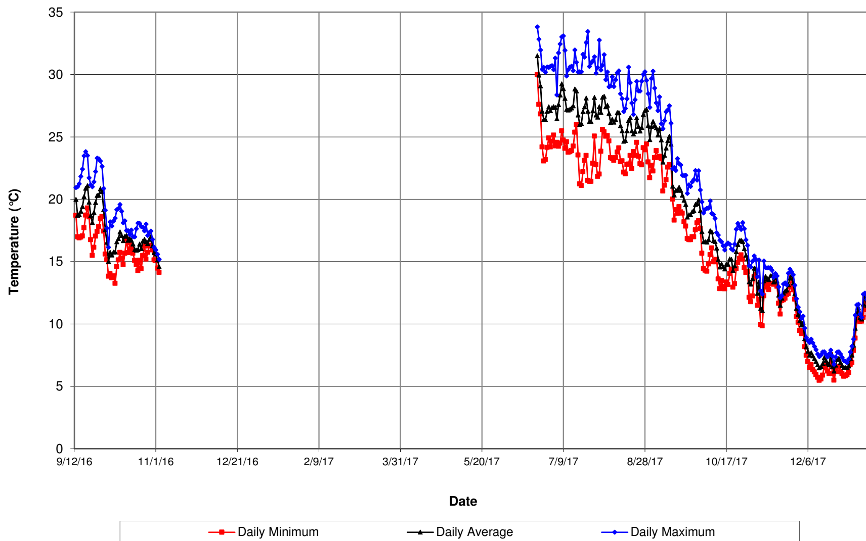
Dry Creek upstream of Bear River Daily Minimum, Average, and Maximum Water Temperature (°C)
