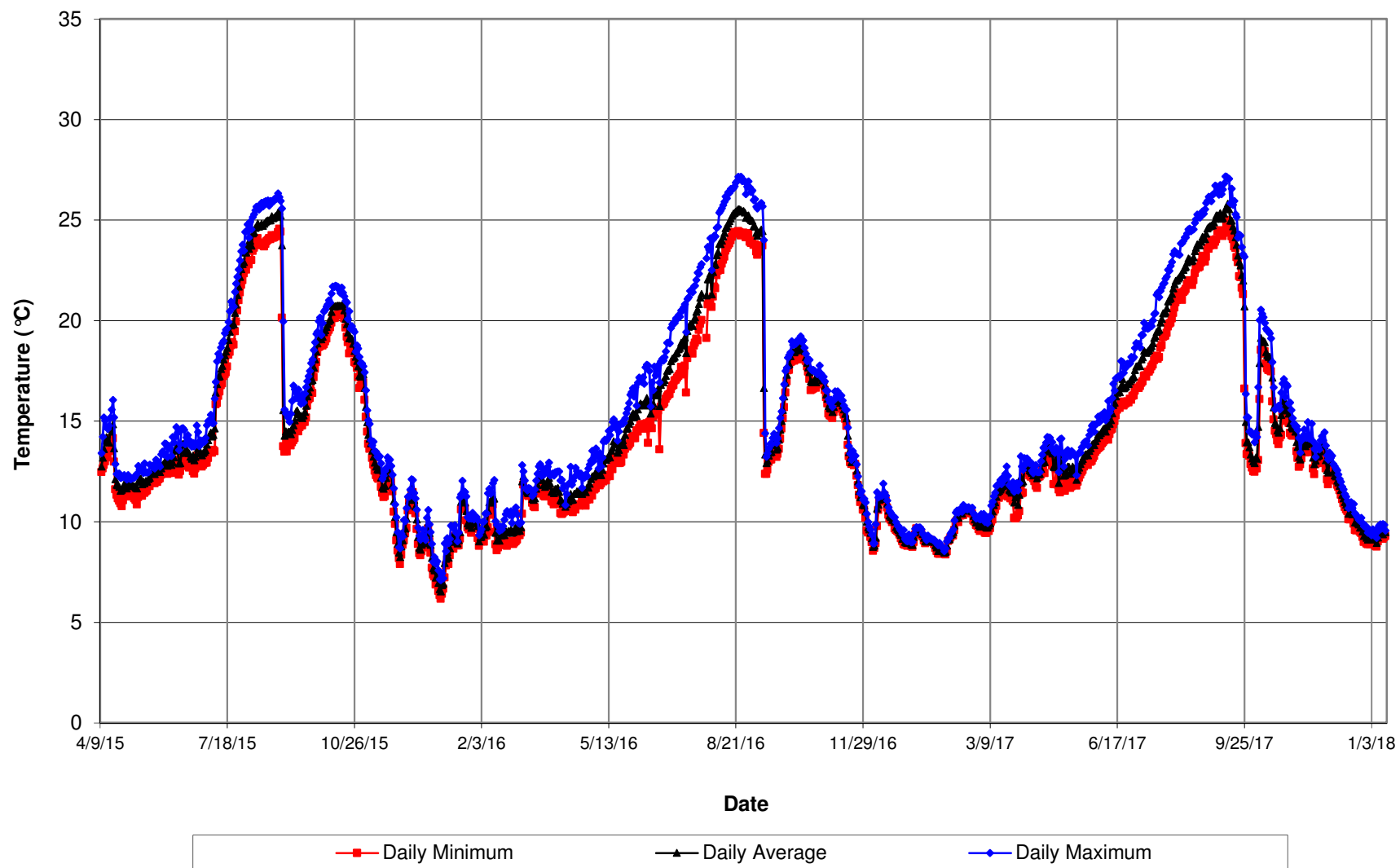
Bear River downstream of Non-Project Diversion Dam Daily Minimum, Average, and Maximum Water Temperature (°C)
