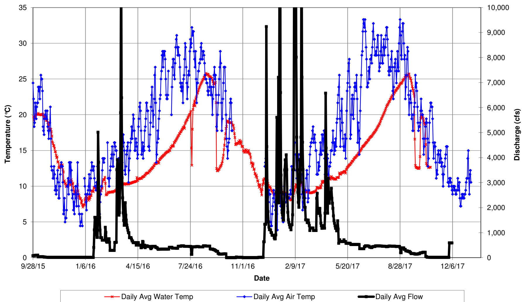
Bear River downstream of Camp Far West Spillway Daily Average Water Temp (°C), Daily Average Air Temp (°C), and Daily Average Flow (cfs) Air Temp at CDEC - CFW, Flow from SSWD Data
