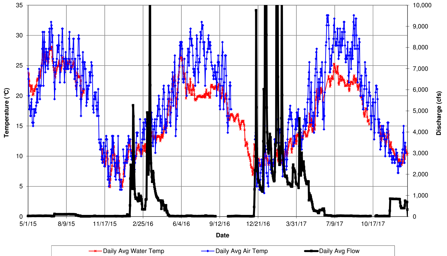
Bear River upstream of Feather River Daily Average Water Temp (°C), Daily Average Air Temp (°C), and Daily Average Flow (cfs) Air Temp at CDEC - CFW, Flow at CDEC - BRW Note: Depending on flows this site can be backwatered by the Feather River
