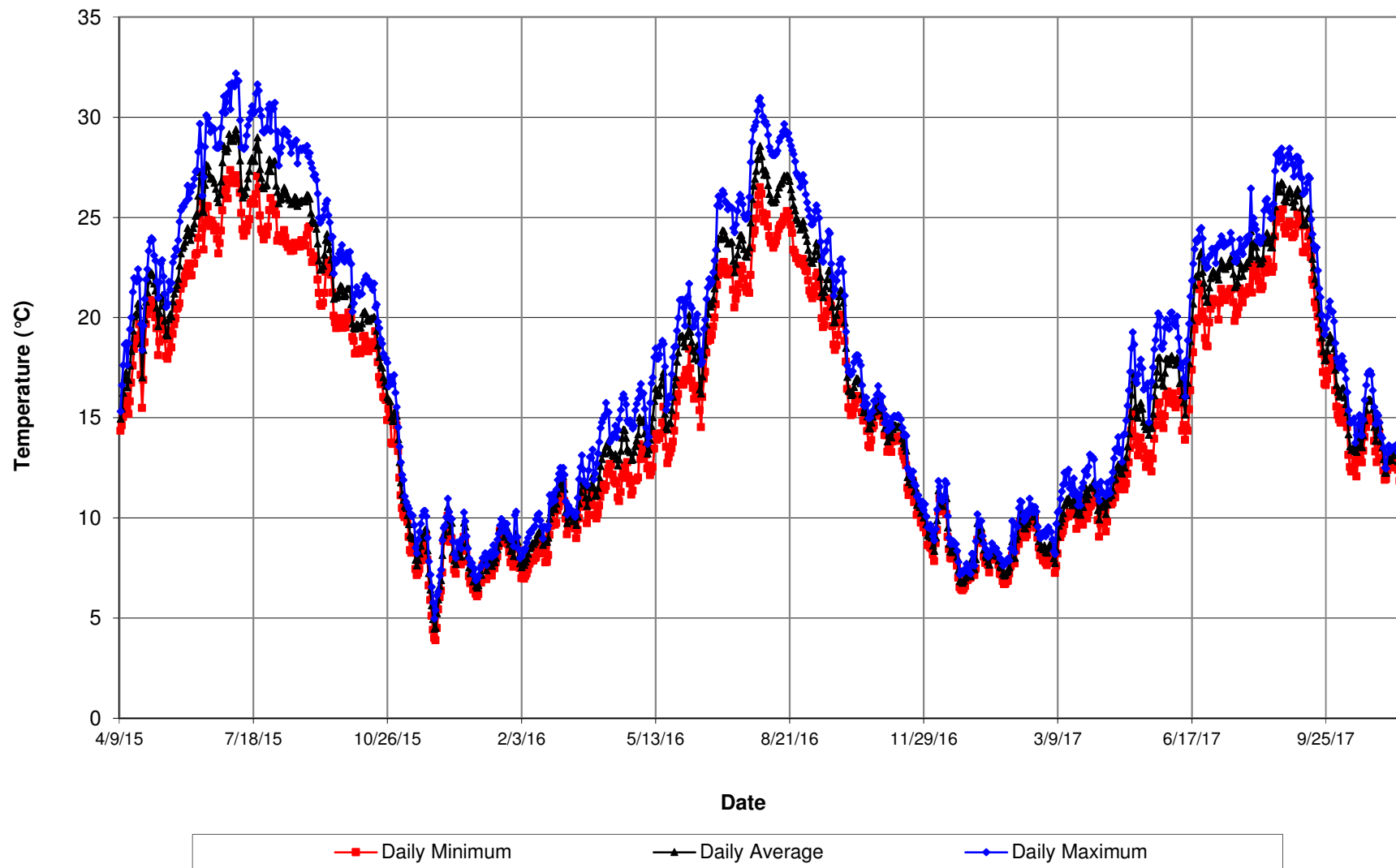
Bear River upstream of Camp Far West Reservoir Daily Minimum, Average, and Maximum Water Temperature (°C)
