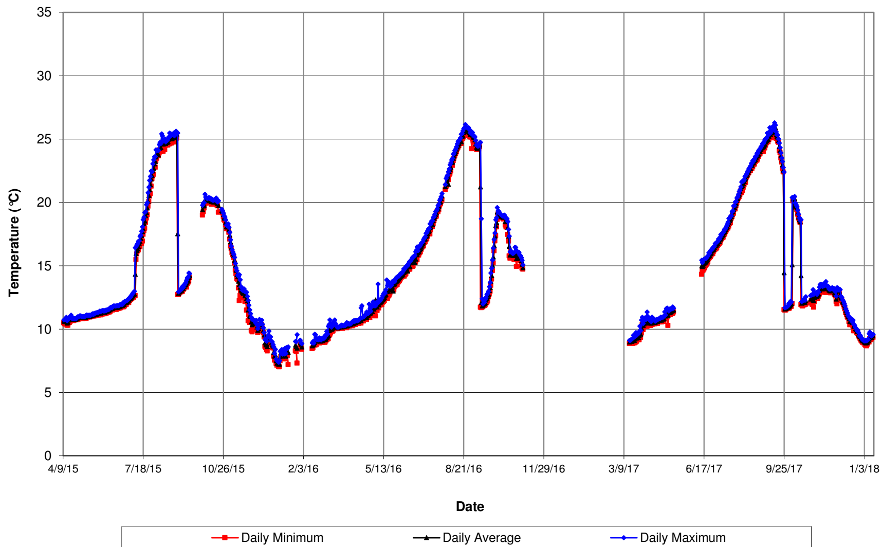
Bear River downstream of Powerhouse Daily Minimum, Average, and Maximum Water Temperature (°C)
