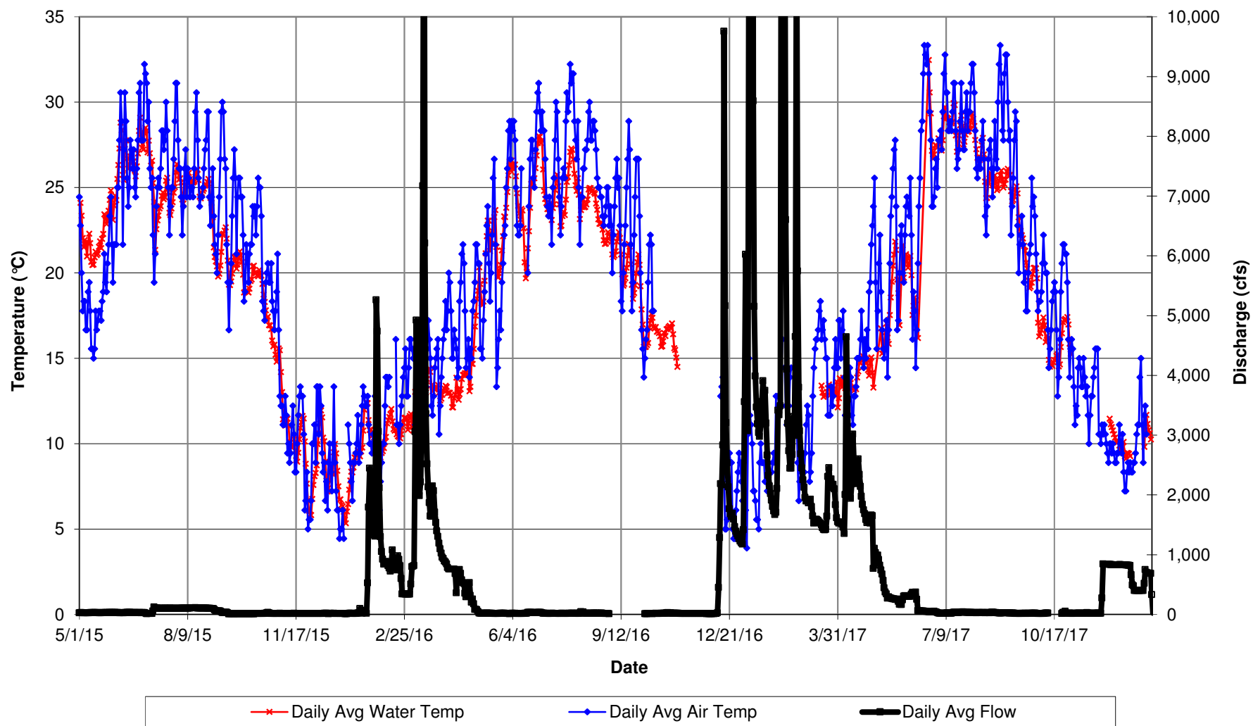
Bear River downstream of Highway 70 Bridge Daily Average Water Temp (°C), Daily Average Air Temp (°C), and Daily Average Flow (cfs) Air Temp at CDEC - CFW, Flow at CDEC - BRW
