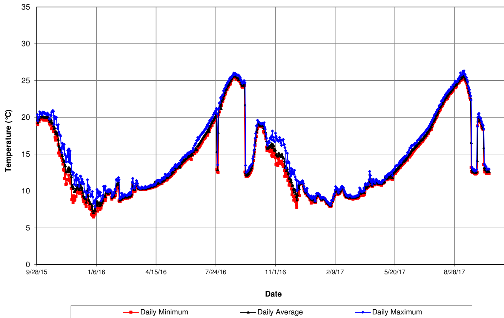
Bear River downstream of Camp Far West Spillway Daily Minimum, Average, and Maximum Water Temperature (°C)
