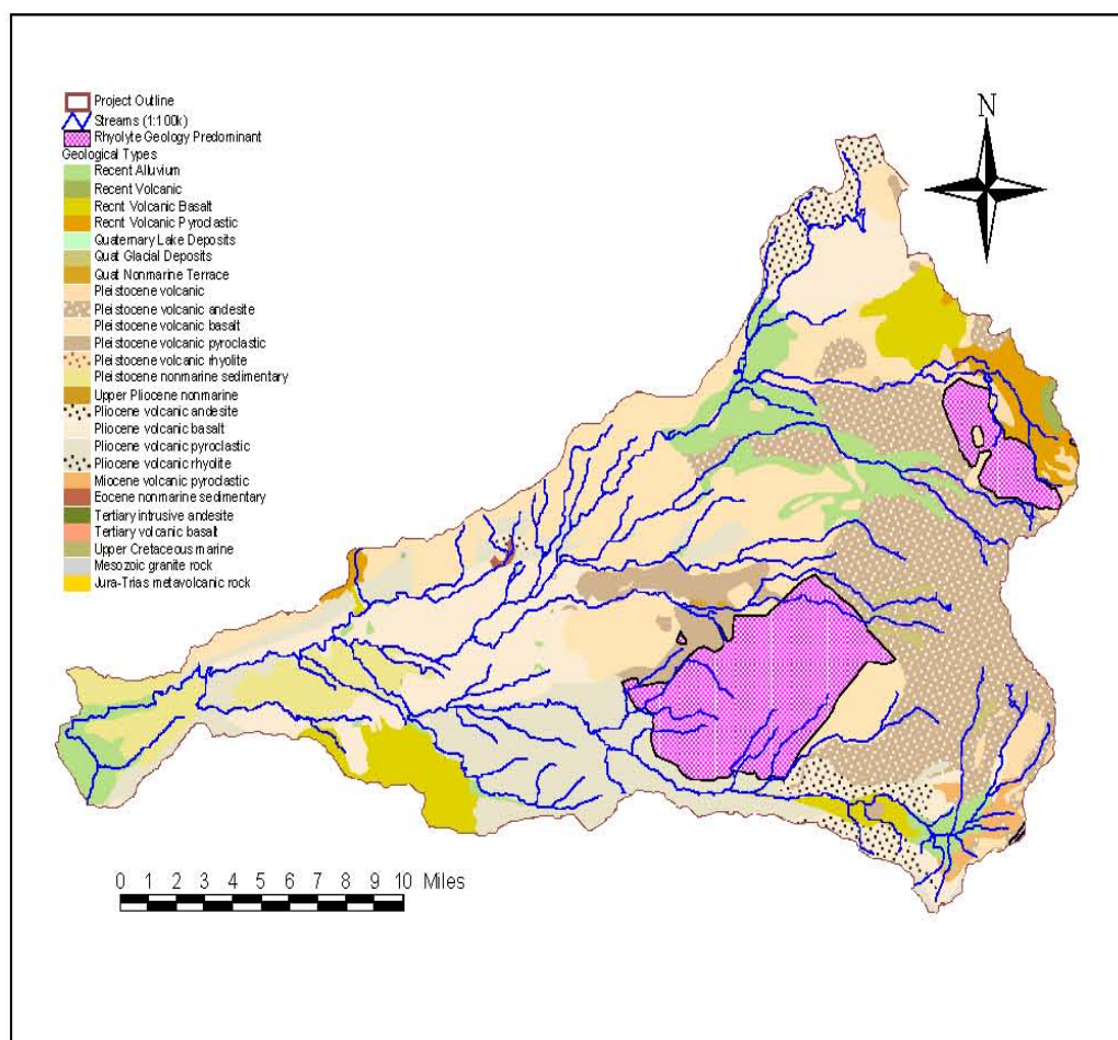
Figure 14. Battle Creek geologic types and location of rhyolitic soils (purple)
